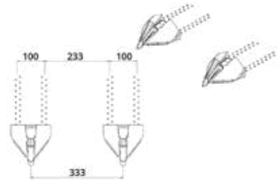
+ DTS 5" DOUBLE ROW SEED BOOT (STANDARD) SWB443
